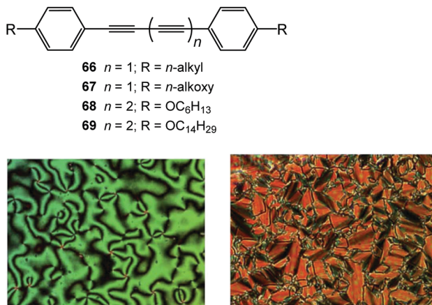
Fig. 25 Structures of 66 – 69 . Polarised-light optical microscopy images of 69 at 130 °C (left) and 117 °C (right). Reproduced from ref. 183 with permission from the Royal Society of Chemistry.
