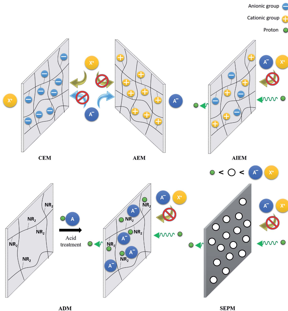
Fig. 10 Selectivity of the different IEMs employed in RFBs.
