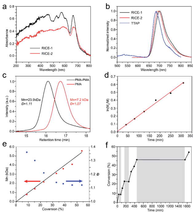
Fig. 3 (a) Solid-state UV-vis spectra of the RICE COFs (b) Fluorescence emission spectra of RICE COFs and TTAP monomer in DMF. Excitation wavelength 460 nm. (c) GPC profiles of PMA and the diblock copolymer (d) first order kinetic plot of the polymerization of MA (DP = 100) (e) M_n and \bar{D} of resulting polymers versus monomer conversion. Black line is theoretical M_n vs. conversion. Blue dots are \bar{D} at different conversion. Red dots are M_n at different conversion. (f) Pulsed-irradiation kinetic experiments. The shaded areas indicate the reaction operated in the dark while the unshaded areas represent the reaction under irradiation.
