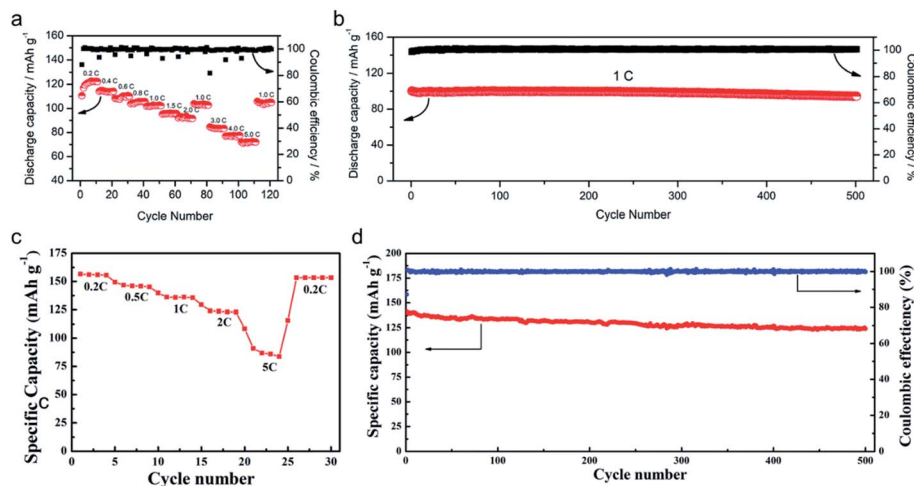
Fig. 18 Practical performances in battery prototypes. (a) Energy capacity of the \text{LiFePO}_4|\text{EVOH-graft-LiCPSI}| \text{electrolyte}|\text{Li} cell at room temperature over many charge/discharge cycles at various C rates. (b) Long term stability at 1C for 500 cycles. (a and b) are reproduced with permission. 157 Copyright 2018, Royal Society of Chemistry. (c) Rate capability of \text{Li}|\text{LiBAMB-PETMP/GBL}|\text{LiFePO}_4 cells. (d) Cycle performance at 1C. (c and d) are reproduced with permission. 158 Copyright 2017, Elsevier.
