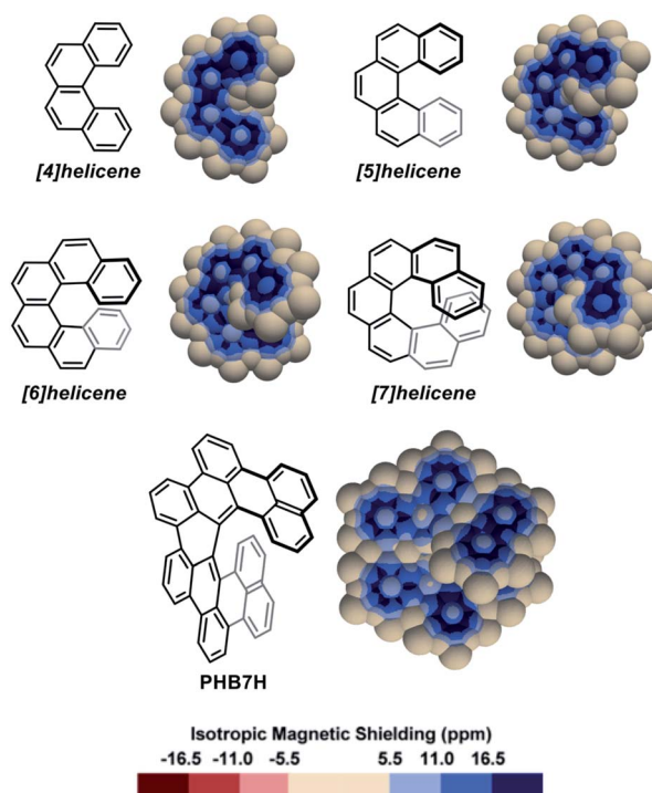
Fig. 2 3D IMS contour maps of [n] helicenes and peri -hexabenzocycloheptatriene (PHB7H) calculated at the B3LYP-GIAO/6-311++G**//B3LYP-D3BJ/def2-SVP level of theory.
