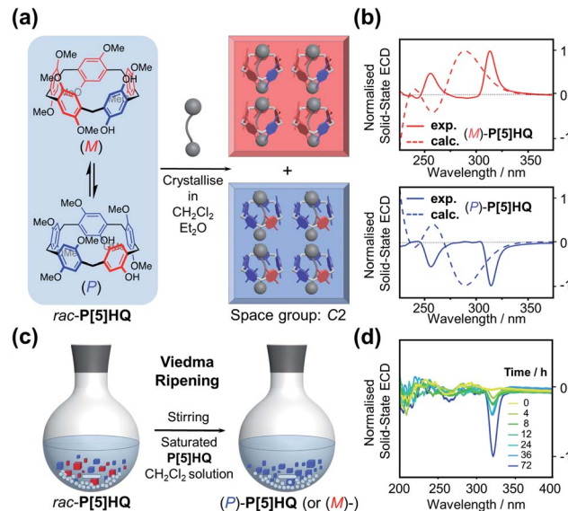
Fig. 2 (a) Schematic representation of the spontaneous resolution of rac-P[5]HQ. The mechanical mixture of enantiomeric crystals can be resolved by triage. (b) Normalised solid-state ECD spectra of randomly handpicked (M)- and (P)-P[5]HQ single crystals (solid lines) and stimulated ECD spectra of (M)- and (P)-P[5]HQ (dashed lines). (c) Schematic representation of Viedma ripening. (d) Normalised solid-state ECD spectra of a near-racemic P[5]HQ sample gradually showing crystal enantiomeric excess during the process of Viedma ripening.
