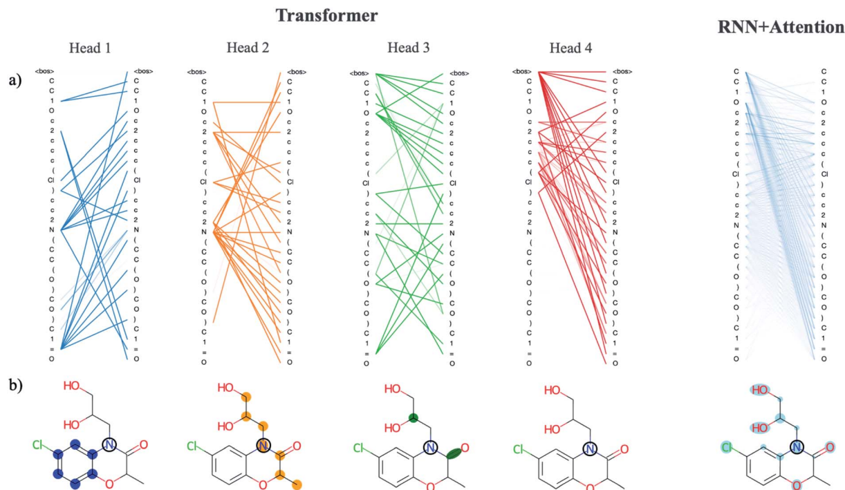
Fig. 4 Analysis of the attention weights of the Trans4x-256 and RNNAttn-256 models when attending to the molecular structure of diproxadol. The full nxn set of weights are plotted for each attention head within the first layer of the encoder (a) using the tensor2tensor library. 57 The lines show how each atom/structural feature within the SMILES string is attending to all other features within the same SMILES string (self-attention). The different patterns that emerge from each head represent a unique set of grammatical rules that the model has learned. We also show the attention of a single N atom within diproxadol (b). This molecule was chosen because it is a representative example of the emergent aggregate grammatical trends. From the perspective of the nitrogen, the transformer model has identified the importance of a nearby aromatic ring (head 1), an aliphatic carbon chain of which the nitrogen is a part of (head 2) and a set of structural features including a carbon branch point and nearby double bond (head 3). The attention of the nitrogen in the RNNAttn-256 model is less focused.
