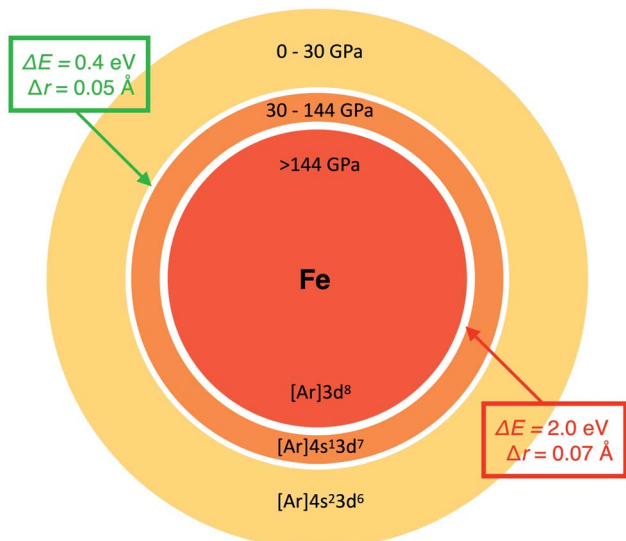
Fig. 3 Example of the relationship between atomic radius and total energy. The size of the Fe atom at different pressures is to scale. White regions correspond to [Ar]4s^23d^6 ( S = 2 ) \rightarrow [Ar]4s^13d^7 ( S = 2 ) and [Ar]4s^13d^7 \rightarrow [Ar]3d^8 ( S = 1 ) ground state configurational transitions predicted at 30 and 144 GPa, respectively.
