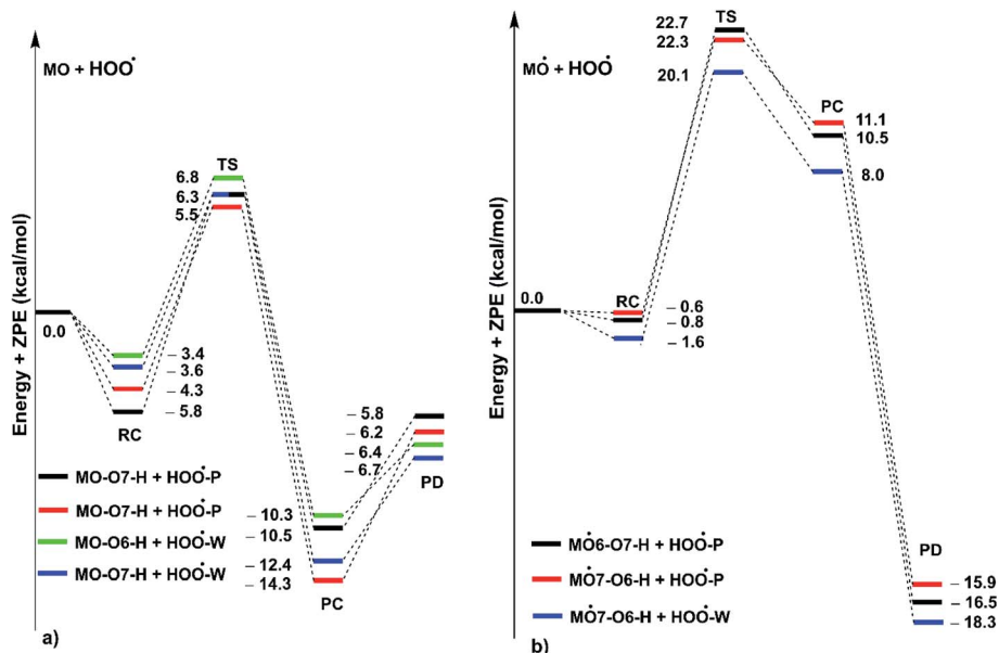
Fig. 5 PES of reactions between MO and HOO • in pentyl ethanoate (P) and water (W) in double processes (a): the first step; (b) the second step; RC: pre-complexes, TS: transition states, PC: post-complexes, PD: products).
