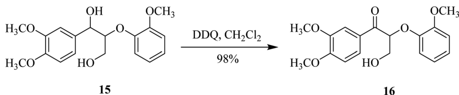
Scheme 7 Selective benzylic oxidation of \beta -O-4 model compound 15 .
