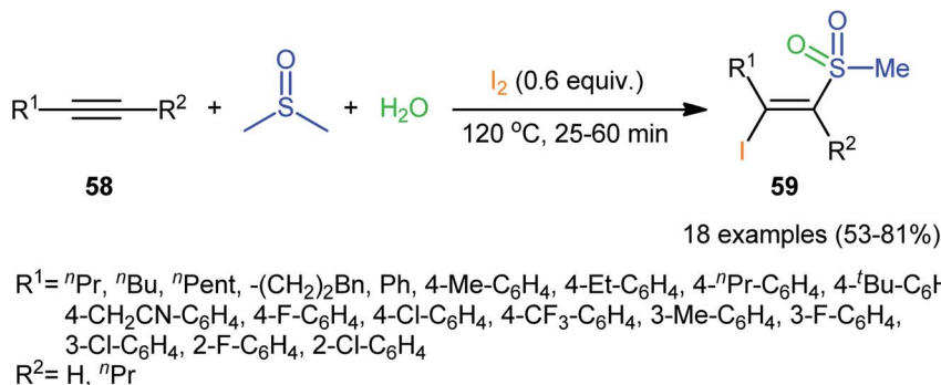
Scheme 26 Catalyst-free four-component synthesis of ( E )- \alpha -iodo- \beta -methylsulfonylalkenes 59 from alkynes 58 , DMSO, I 2 , and H 2 O.
