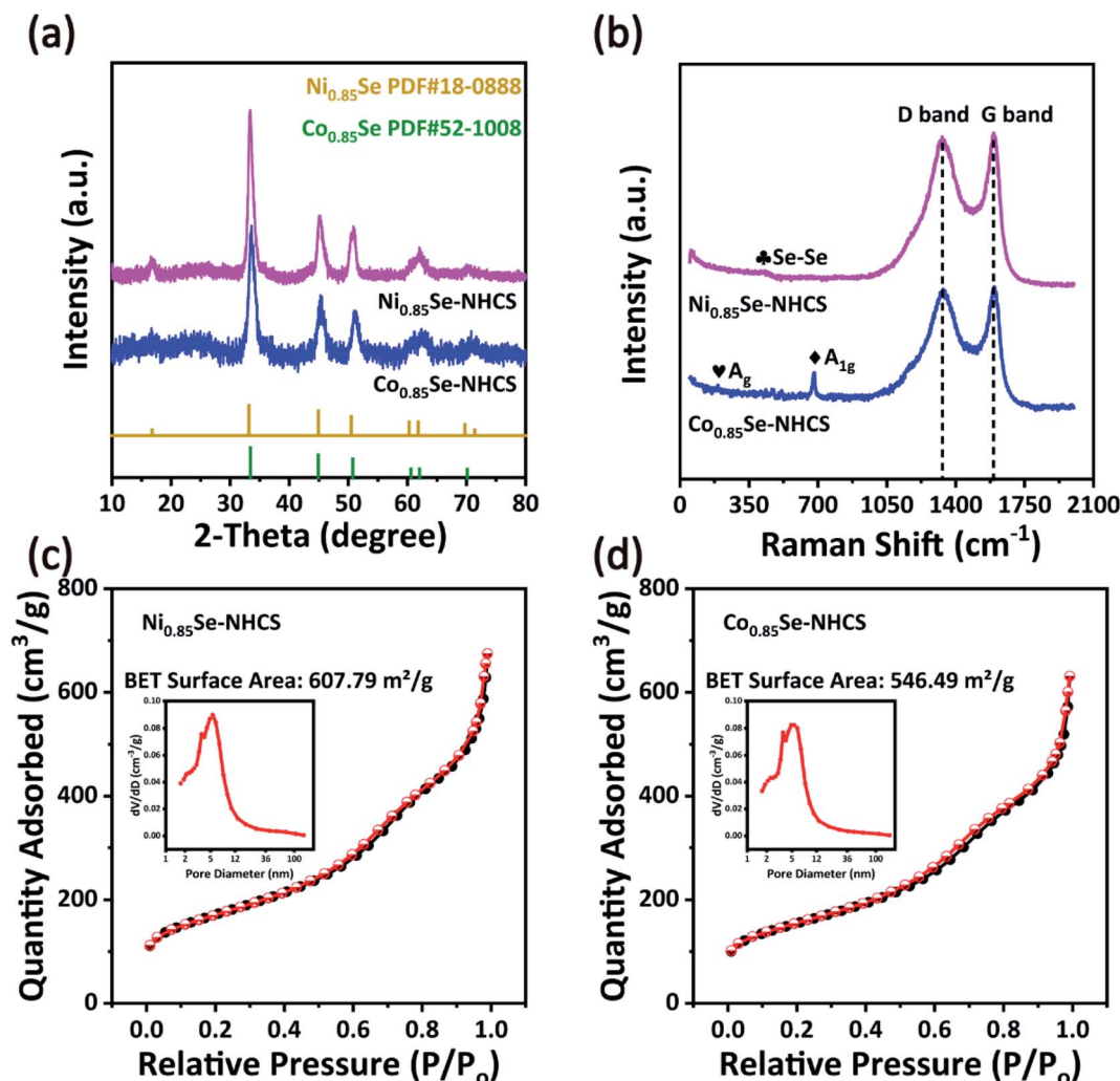
Fig. 3 (a) The XRD patterns and (b) Raman patterns of \text{Ni}_{0.85}\text{Se} -NHCS and \text{Co}_{0.85}\text{Se} -NHCS. (c) \text{N}_2 adsorption/desorption isotherms of \text{Ni}_{0.85}\text{Se} -NHCS (inset: pore size distribution) and (d) \text{N}_2 adsorption/desorption isotherms of \text{Co}_{0.85}\text{Se} -NHCS (inset: pore size distribution).
