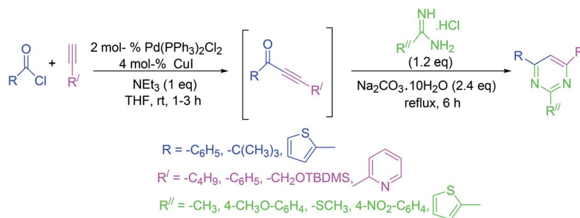
Scheme 13 One-pot pyrimidine synthesis by the pairing of acid chlorides and terminal alkynes.
