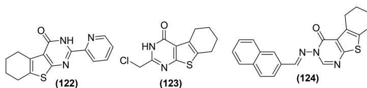
Fig. 36 Chemical structures of selected tetrahydrobenzo[4,5]thieno[2,3- d ]pyrimidine derivatives ( 122–124 ).
