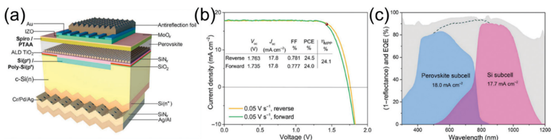
Fig. 7 (a) Scheme of the interlayer-free monolithic perovskite–c-Si tandem solar cell. (b) J-V curve of the tandem device with both reverse and forward scanning at 0.05\text{ V s}^{-1} based on heterojunction poly-Si subcell. (c) Absorbance (1-reflectance) of the tandem device (gray), EQE of the perovskite top cell (blue), and the c-Si bottom subcell (pink). 29
