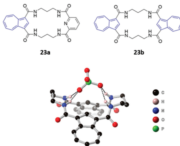
Fig. 10 (Top) Structures of tetraamide macrocyclic anion receptors with azulene units shown in blue. (Bottom) Crystal structure of 23b · \text{H}_2\text{PO}_4^- , with hydrogen bonds between the receptor amide groups and \text{H}_2\text{PO}_4^- shown as dashed lines. All other hydrogen atoms have been omitted for clarity. K_a(\text{H}_2\text{PO}_4^-) = 4800 \text{ M}^{-1} for 23a and >10^4 \text{ M}^{-1} for 23b in 9 : 1 DMSO/MeOH.
