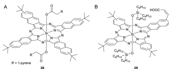
Instead of using two distinct SiPc and SiNc dyes, Sellinger et al. developed a hybrid SiNcPc, 29 bearing a mononaphthalo triphthalo cyanine core and investigated its photosensitizing properties in a DSSC (Fig. 11B). 118 A vinyl group was introduced in the mononaphthalo ring to establish conjugation with an anchoring carboxylic acid unit. The hybrid dye, 29 exhibited high solubility, high extinction coefficients and desirable energy levels. The integration of 29 in solar devices resulted in high photocurrents of 19.0 A cm -2 and a total efficiency of 4.5% (Table 1).
