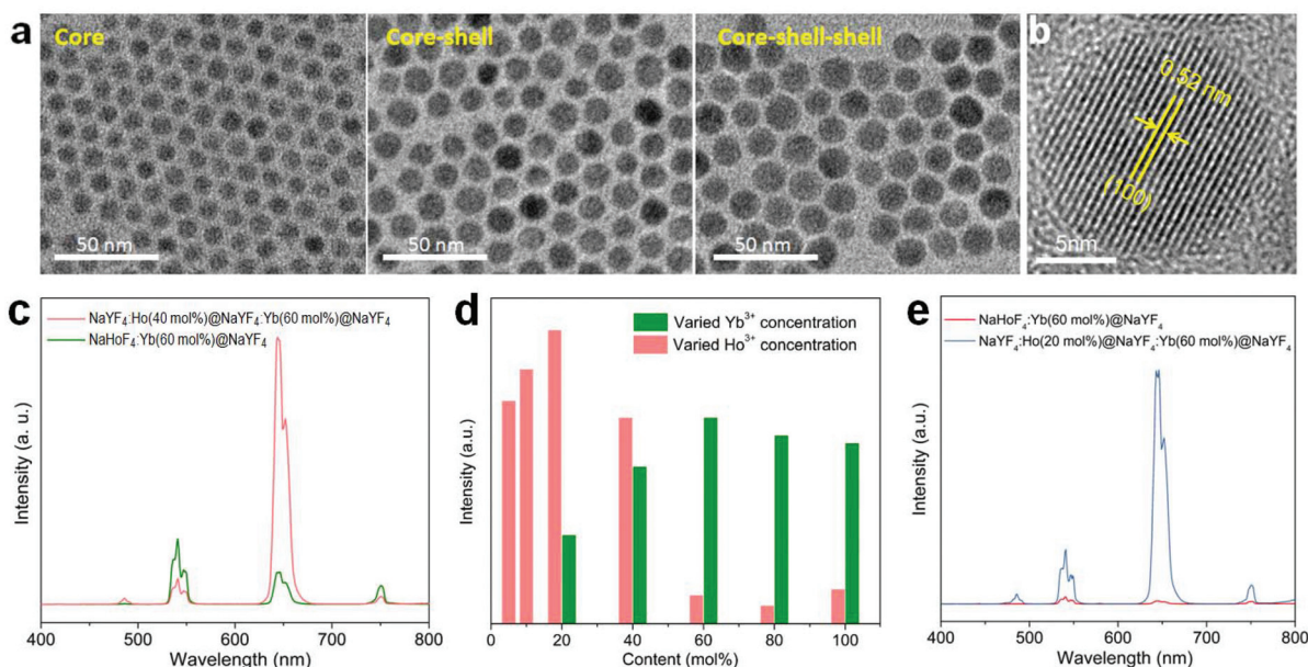
Fig. 3 (a) TEM images of the NaYF 4 :Ho(40 mol%) core, NaYF 4 :Ho(40 mol%)@NaYF 4 :Yb(60 mol%) core-shell, and NaYF 4 :Ho(40 mol%)@NaYF 4 :Yb(60 mol%)@NaYF 4 core-shell-shell nanoparticles. (b) The high-resolution TEM image of the core-shell-shell nanoparticles. (c) A comparison of the upconversion emission spectra of as-prepared NaYF 4 :Ho(40 mol%)@NaYF 4 :Yb(60 mol%)@NaYF 4 core-shell-shell and NaHoF 4 :Yb(60 mol%)@NaYF 4 core-shell nanoparticles under 980 nm excitation. (d) Dependence of the overall upconversion emission intensity of the NaYF 4 :Ho(5–100 mol%)@NaYF 4 :Yb(20–100 mol%)@NaYF 4 core-shell-shell nanoparticles with a tuning of the concentrations of Ho 3+ in the core and Yb 3+ in the interlayer, respectively. (e) Comparative upconversion emission spectra from the optimized NaYF 4 :Ho(20 mol%)@NaYF 4 :Yb(60 mol%)@NaYF 4 core-shell-shell nanoparticles and NaHoF 4 :Yb(60 mol%)@NaYF 4 core-shell nanoparticles under identical measurement conditions.
