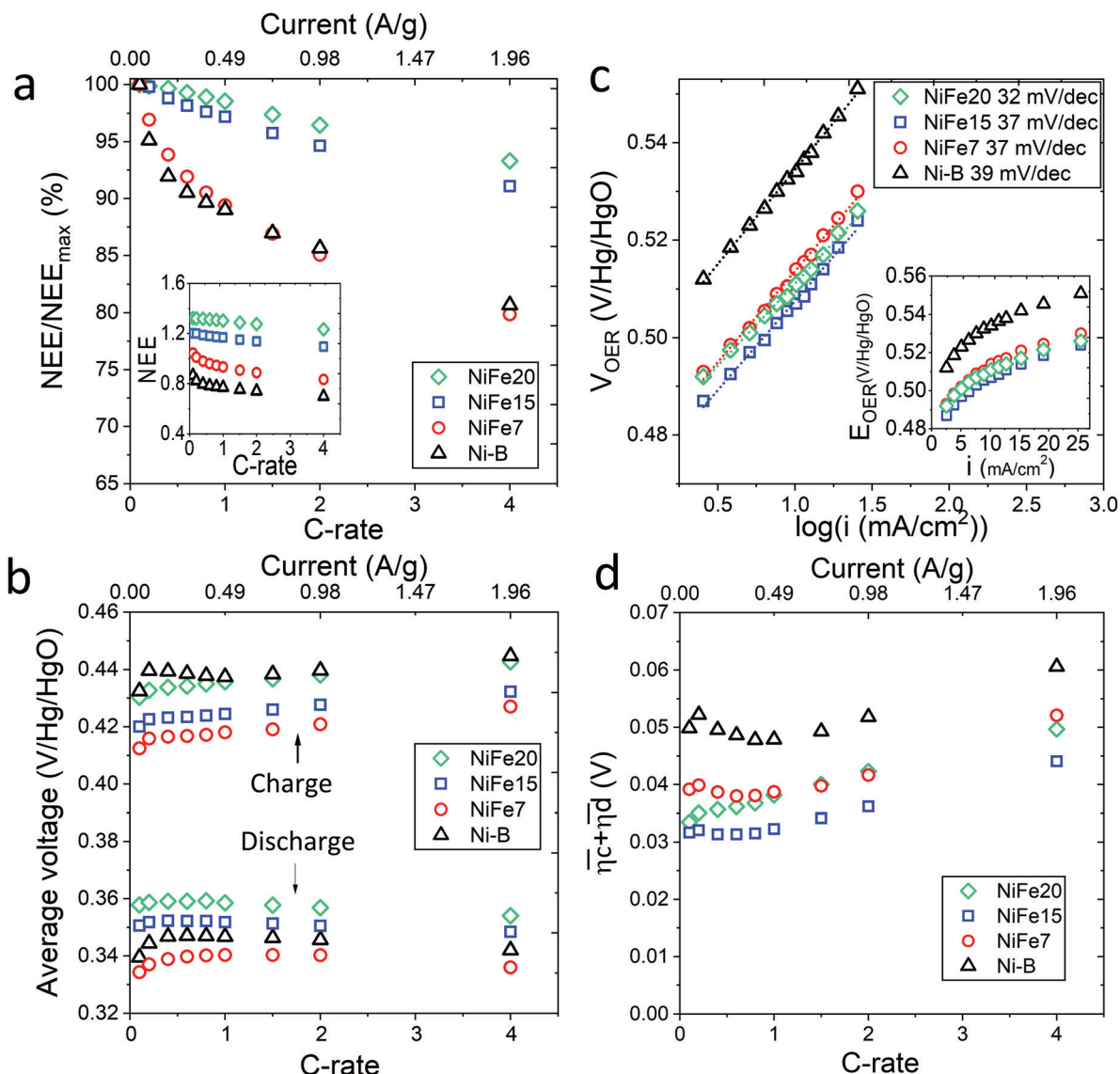
Fig. 4 High rate performances of \beta -Ni(OH) _2 and LDH-Fe-Ni(OH) _2 materials. (a) Evolution of the discharge capacity with the C-rate represented as the ratio of the discharge capacity to the discharge capacity at a C-rate of 0.1C and, in the inset, as NEE, (b) average voltage of the (dis)charge curve for the different C-rates, (c) iR corrected OER Tafel plots and, in the inset, evolution of V_{\text{OER}} with current density, and (d) sum of the kinetic overpotentials for different C-rates.
