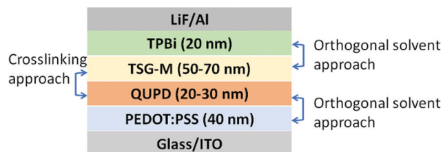
Fig. 16 Schematic of OLEDs structure with four organic layers. QUPD is N,N -bis(4-(6-((3-ethyloxy)hexyloxy)phenyl)- N,N -bis(4-methoxyphenyl)biphenyl-4,4-diamine, TSG-M is green emitter. (reproduced from the ref. 95).
