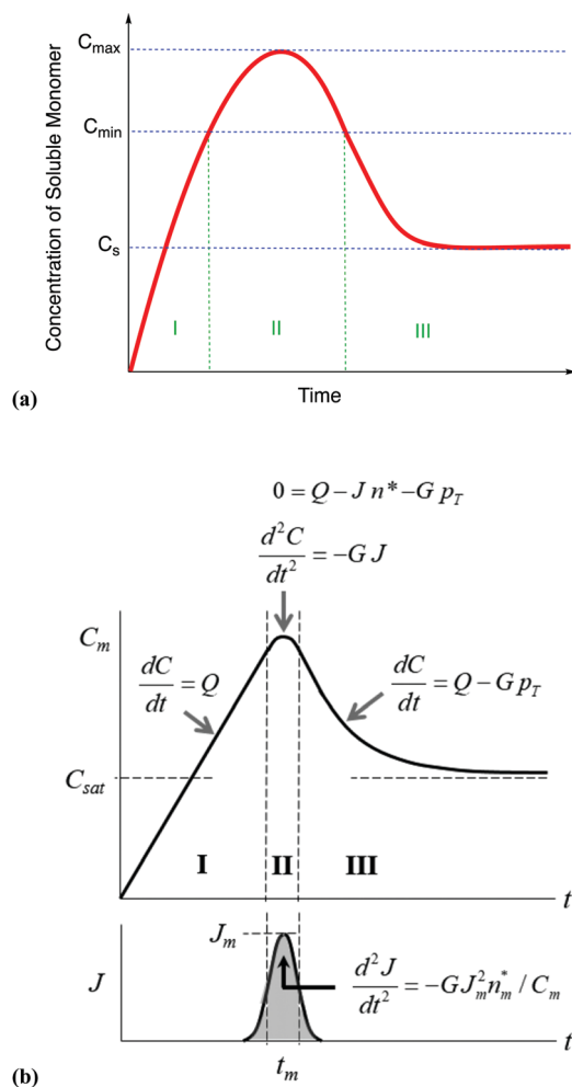
Fig. 7 (a) A schematic illustration of the 1950 hypothesis in picture form for the formation of colloidal particles, 1 originally for soluble monomer, S , in the case of sulfur sol formation, ( S ), (a) is representative of what one finds in the literature, including what we have presented elsewhere, 2 although LaMer's actual diagram 2 in the original 1950 paper has a more linear initial rise. The hypothetical curve in (a) shows qualitatively the variation of soluble monomer concentration versus time during the whole formation process. C_s is the saturation concentration (of the soluble monomer), C_{\min} is the hypothetical minimum supersaturation for the nucleation, and C_{\max} is the hypothetical limiting supersaturation, postulated stage I: formation of soluble monomer in solution. Postulated stage II: nucleation from the solution when the concentration of soluble monomer is higher than the critical supersaturation level C_{\min} —as typically presented, albeit not shown as truly postulated “effectively infinite rate, burst nucleation”. 1 Postulated stage III: growth by diffusion when the supersaturation concentration is lower than C_{\min} , but higher than C_s . It is critical to note that, in the intervening nearly 70 years, and despite the widespread reproduction and quoting of this figure, no such experimental time dependence of soluble sulfur monomer has ever been published, at least that we have been able to find from an exhaustive literature search. Reproduced with permission, including the figure caption, from ref. 2. Copyright 2019 American Chemical Society. (b) The more quantitative version of the classic 1950 figure 1 from B. Peters et al. , that they describe by “each stage of a LaMer burst nucleation process is described by different equations that relate the solution concentration C , the nucleation rate J , the number of nuclei p_T , the growth rate G , and the nucleus size n^* .” 103 (b) Also more faithfully reproduces the initial linear rise given in LaMer's classic figure (Fig. 1 in the 1950 paper. 1 ) Reproduced with permission from ref. 103. Copyright 2017 American Chemical Society.
