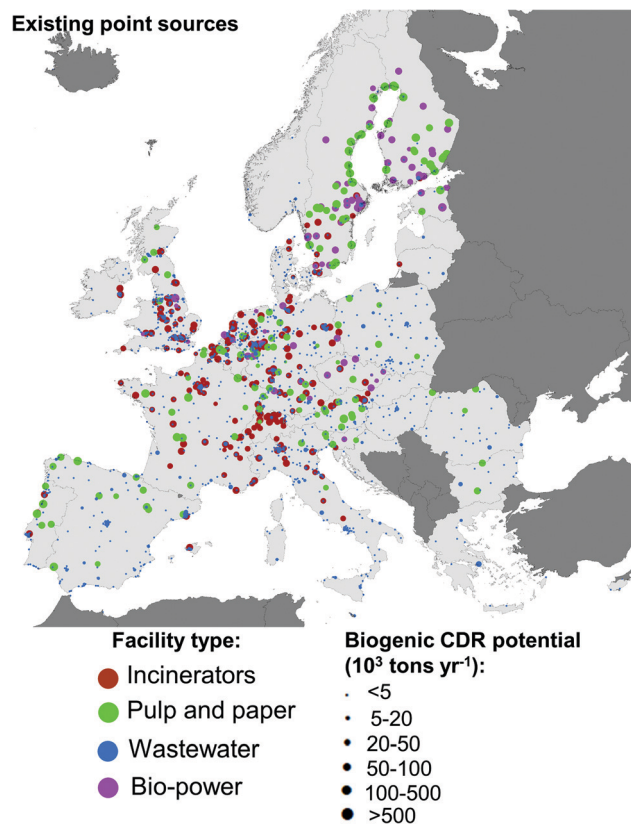
Fig. 2 Geospatial distribution of biogenic carbon dioxide removal potential from existing point sources in Europe in 2018 (see ESI † ). The figure shows incinerators, pulp and paper, and bio-power facilities emitting more than 0.1 Mtons CO 2 per year, 54 and wastewater treatment plants processing more than 100 000 population equivalent of wastewater per day. 53
