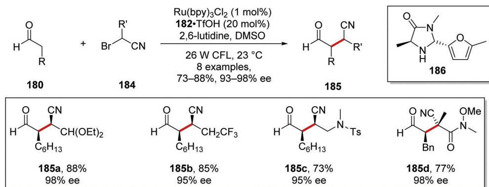
Scheme 43 Scope of the α-bromonitriles 184 .
