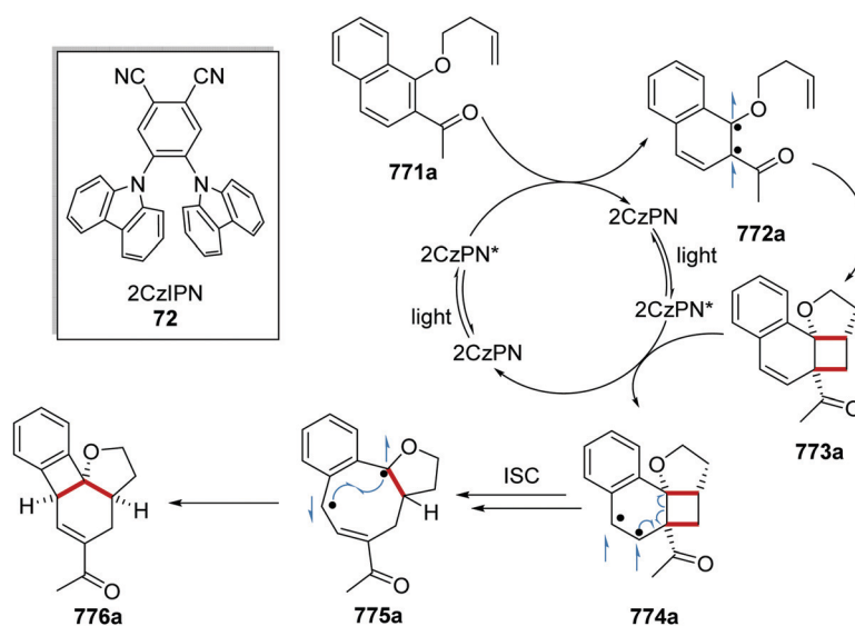
Scheme 210 Dearomatizing rearrangements of naphthol derivative 771a .
