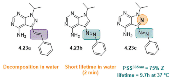
Fig. 51 Inhibitors of RET transmembrane tyrosine kinase receptor, illustrating the effect of a different switch system (stilbene 4.23a vs. azobenzene 4.23b and c ) and an additional heteroatom ( 4.23b and c ) on the (photo)chemical properties in aqueous solutions.
