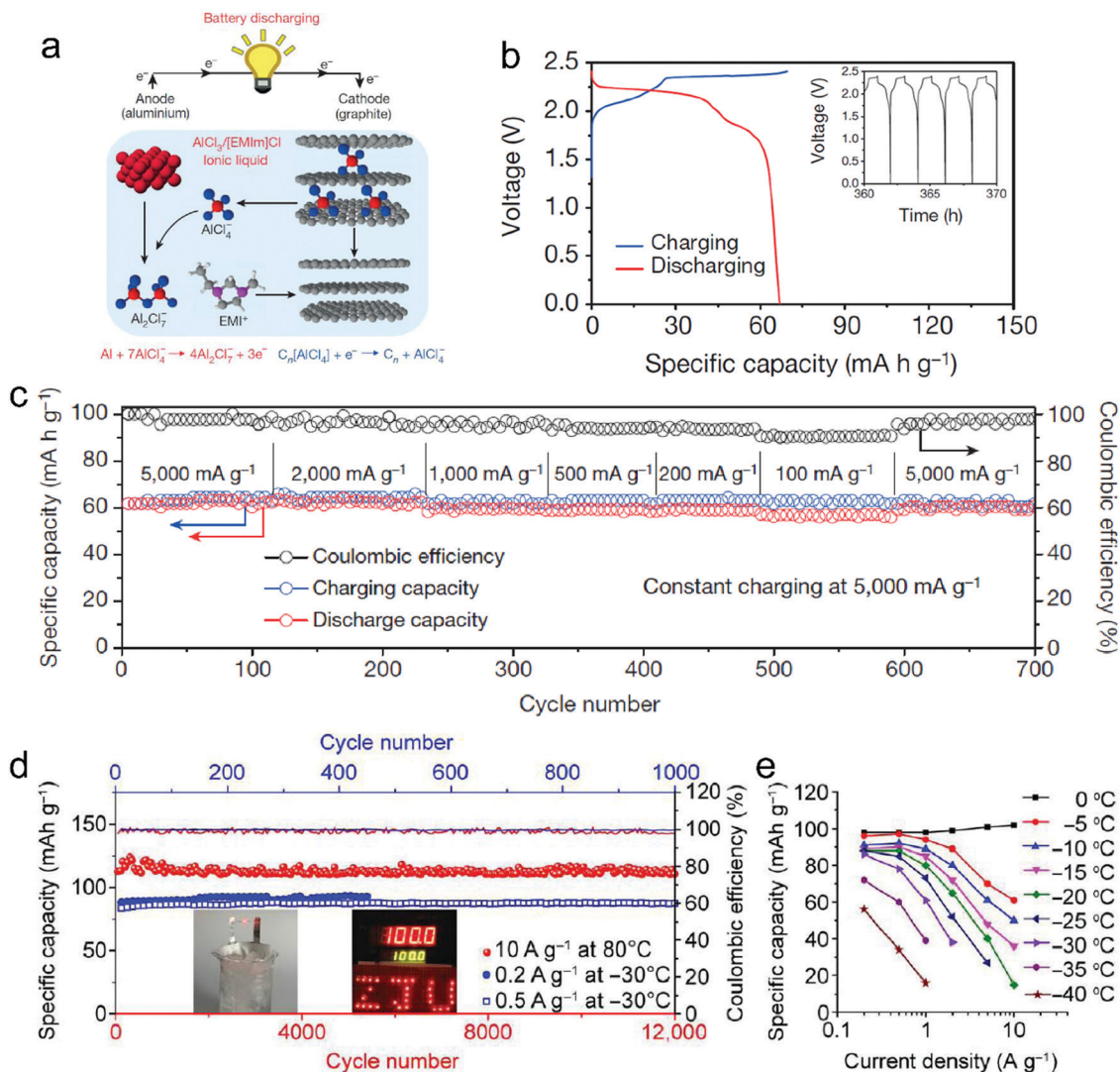
Fig. 29 (a) Schematic drawing of the Al/graphite cell during discharge, using the optimal composition of the AlCl 3 /EMImCl IL electrolyte. (b) Galvanostatic charge and discharge curves of an Al/pyrolytic graphite (PG) Swagelok cell at a current density of 66 mA g -1 . Inset, charge and discharge cycles. (c) An Al/graphitic-foam pouch cell charging at 5000 mA g -1 and discharging at current densities ranging from 100 to 5000 mA g -1 . Reproduced from ref. 170 with permission from Springer Nature. (d) Stable cycling of the GF-HC cathode at 80 °C (red, 12 000 cycles) and -30 °C (blue, 1000 cycles). Inset: Al-GB soft pack cells successfully igniting LED lights in an ice-salt bath and a 100 °C oven. (e) Summary of specific capacities and rate capability of the GF-HC cathode at different temperatures below 0 °C. Reproduced from ref. 169 with permission from AAAS.
