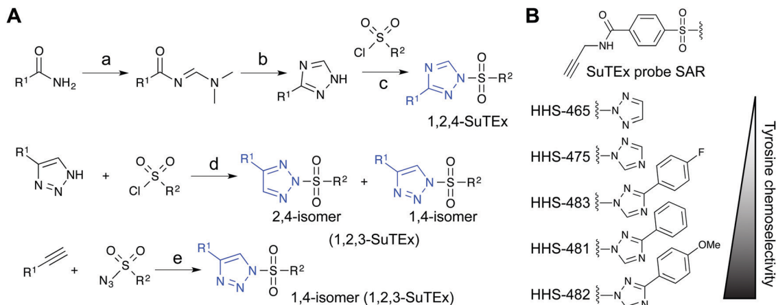
Fig. 4 Synthetic routes for generating triazole diversity for developing SuTE ABPs and ligands. (A) Examples of synthetic routes to generate 1,2,3- and 1,2,4-triazole chemical diversity for developing SuTE ABPs and ligands. The following experimental conditions are used for the synthetic reactions shown: (a) DMF–DMA, 120 °C, 3 hours; (b) Hydrazine, acetic acid, 90 °C, 1.5 hours; (c) ethanol; (d) THF/Et 3 N room temperature, overnight, 1.1 equivalents triazole; (e) toluene, copper(i) thiophene-2-carboxylate (CuTC 175 ), 12–48 hours, 1 : 1 ratio of alkyne and azide. (B) SuTE ABPs with modifications on the triazolide LG. SuTE ABPs containing the 1,2,4-triazolide LG show improved specificity for tyrosine compared with lysine modifications on protein sites and this chemoselectivity can be further augmented with functional group modifications as shown.
