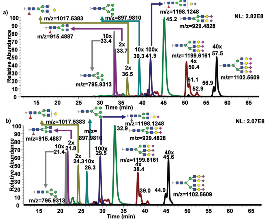
Fig. 3 Effects of higher flow rate for the permethylated glycan analysis using 50 cm \mu PAC. EIC of permethylated N -glycans derived from human blood serum using \mu PAC 50 cm at (a) 300 \text{ nL min}^{-1} flow rate and (b) 600 \text{ nL min}^{-1} . There are noticeable changes in retention time due to the increase in flow rate. Zoom factors such as "10x" indicate zoom in y-axis.
