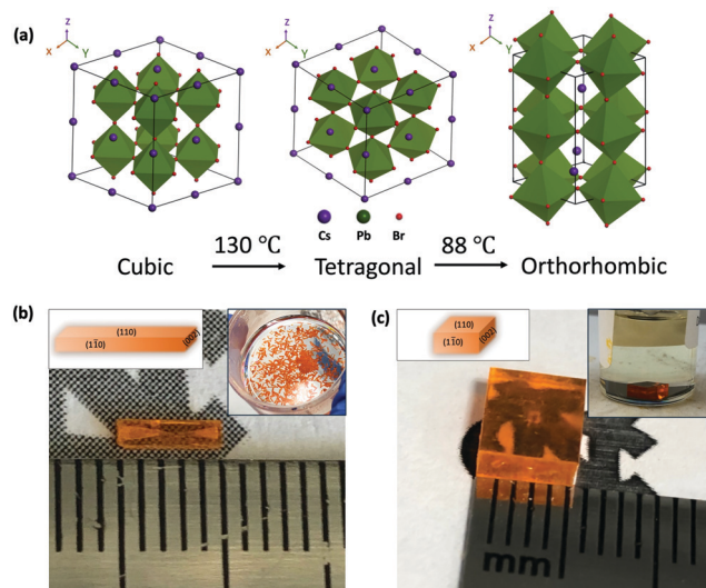
Fig. 1 (a) \text{CsPbBr}_3 structure at different temperature. The transition from cubic to tetragonal happens at 130^\circ\text{C} , and transition from tetragonal to orthorhombic happens at 88^\circ\text{C} . (b) Bar shape \text{CsPbBr}_3 single crystal grown without CB. The left inset indicates the miller indices of each surface, and the right inset is the photograph of crystals in solution. (c) Cuboid shape \text{CsPbBr}_3 single crystal grown with CB. The left inset indicates the miller indices of each surface, the right inset is the photograph of crystals in solution, and the bottom of the vial is a Si-wafer to make a flat bottom.
