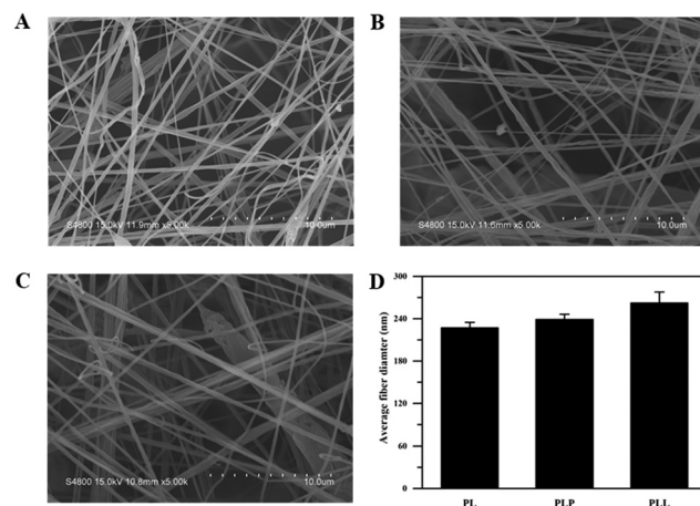
Fig. 2 SEM micrographs of the nanofibrous films: (A) PL film, (B) PLP film, (C) PLL film, and (D) the average nanofiber diameters of the films (PL, PLP and PLL).
