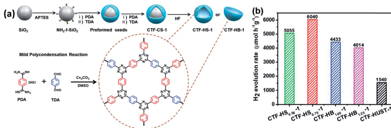
Fig. 10 (a) The schematic synthetic route of CTF-CS-1, where CS represents the \text{NH}_2 -f- \text{SiO}_2 @CTF-HUST-1 core-shell structure, HS is the hollow sphere morphology and HB is the hollow-bowl-like structure morphology. (b) HER of the studied hollow CTFs. Reprinted from ref. 72 with the permission of John Wiley and Sons, Copyright 2019.
