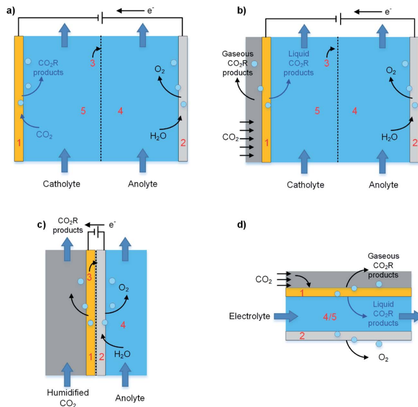
Fig. 5 Schematic of CO 2 electrolyzer in flow-cell configurations (a and b) liquid-fed electrolyzer, (c) vapor-fed electrolyzer and (d) microfluidic reactor. The main cell components are labelled as (1) cathode, (2) anode, (3) separator or ion-exchange membrane which could be a cation exchange membrane, anion exchange membrane, or a bipolar membrane, (4) anolyte, and (5) catholyte.
