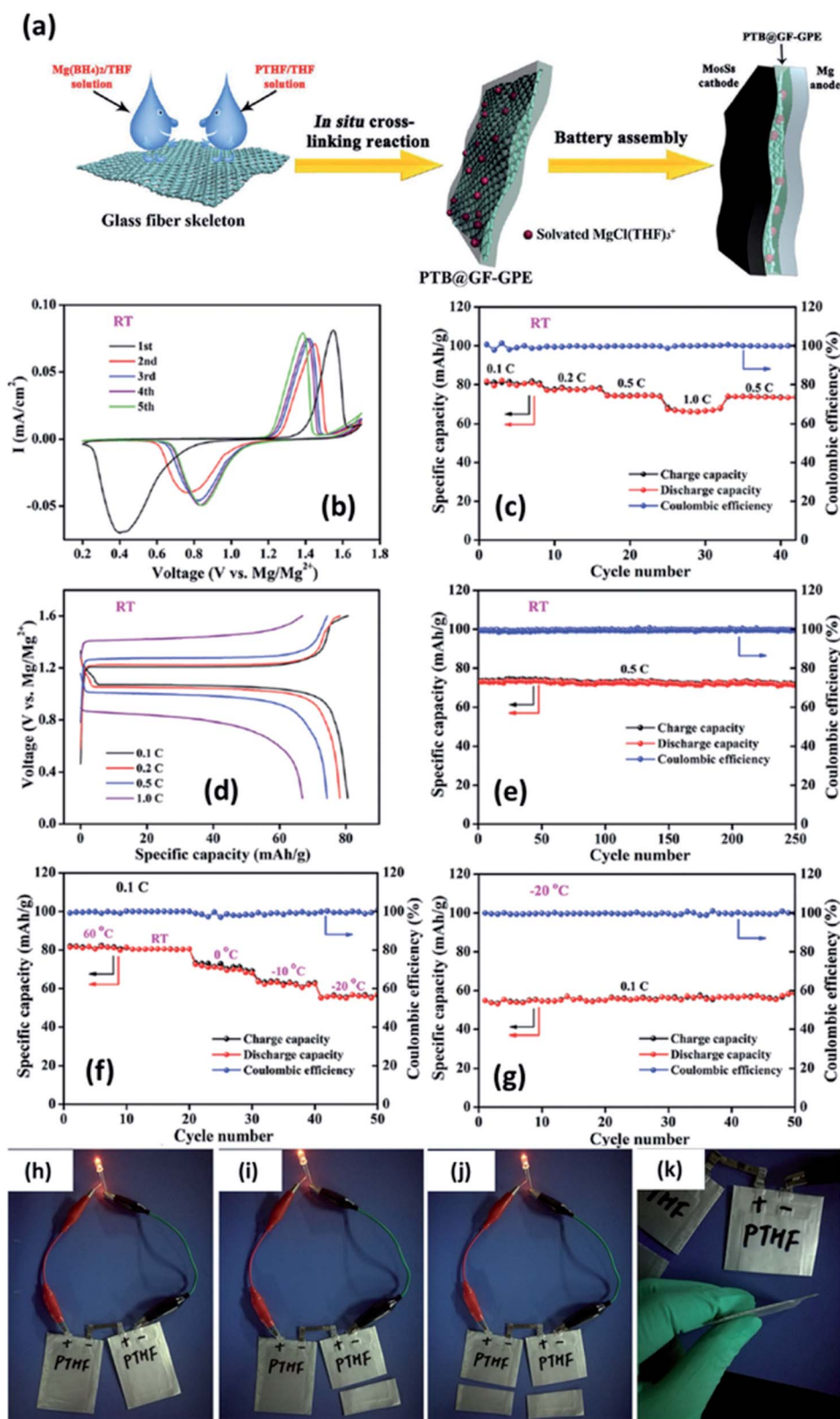
Fig. 11 (a) Schematic of the synthesis of a GPE of borohydride–polytetrahydrofuran impregnated in a glass fiber. Electrochemical characterization of a \text{Mo}_6\text{S}_8/\text{GPE}/\text{Mg} cell at room temperature (b–e) and between 60 and -20 °C (f–g). Lighting an LED using a soft-package \text{Mo}_6\text{S}_8/\text{GPE}/\text{Mg} battery (h–k). Reproduced from ref. 147 with permission, copyright 2019, Wiley.
