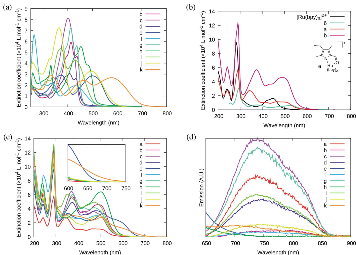
Fig. 1 UV/Vis absorption spectra of (a) ligands 3b–k ; (b) previously reported 6 and [Ru(bpy) 3 ] 2+ as reference complexes for mononuclear 4a and bis[Ru(II)-pyrrolide] triad 4b ; and (c) mononuclear 4a and bis[Ru(II)-pyrrolide] triads 4b–k . (d) Phosphorescence emission spectra for mononuclear 4a and bis[Ru(II)-pyrrolide] triads 4b–k (collected in Ar using \lambda_{\text{ex max}} ). Absorption and emission spectra were collected on the PF 6 − salts of the complexes (5 \mu\text{M} ) in MeCN.
