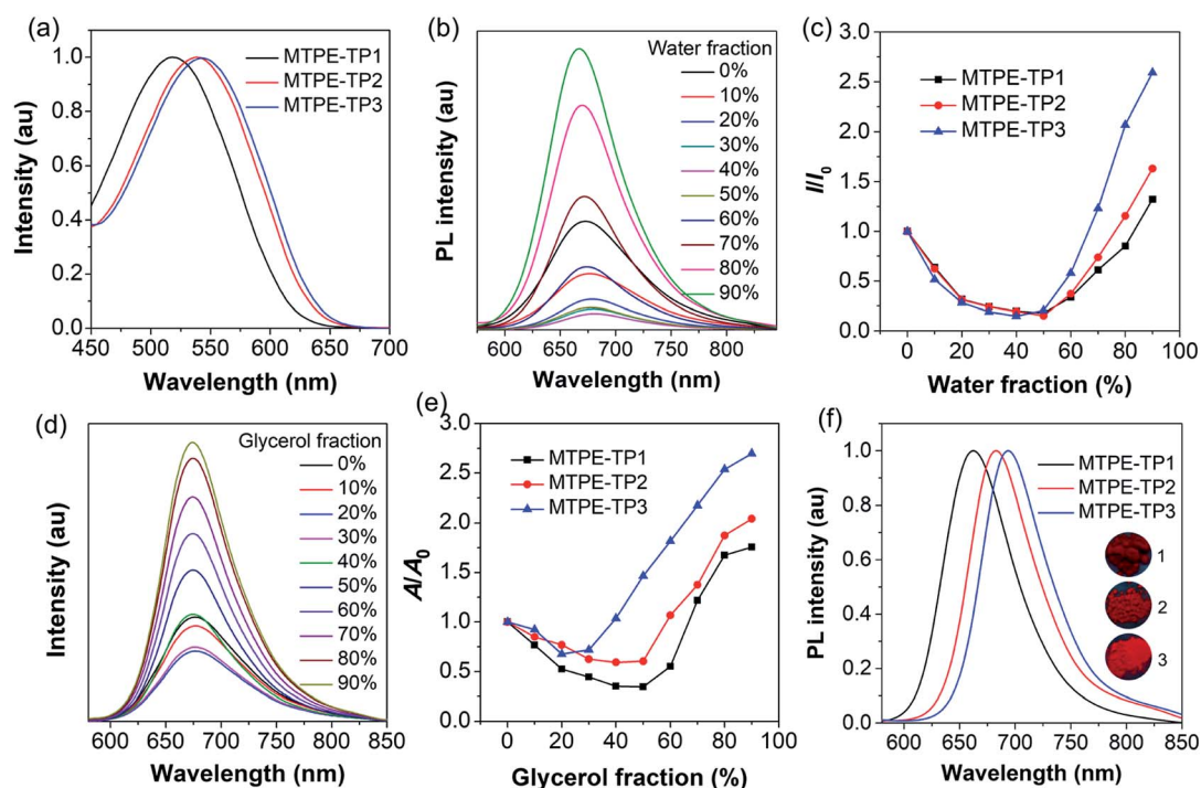
Fig. 2 (a) Absorption spectra of MTPE-TP1-3 in DMSO (10 -5 M). (b) PL spectra of MTPE-TP3 and (c) plot of the PL peak intensity versus water fraction ( f w ) in DMSO/water mixtures (10 -5 M). I 0 and I represent the PL intensities of the compounds in pure DMSO ( f w = 0) and DMSO/water mixtures with specific f w s, respectively. (d) PL spectra of MTPE-TP3 and (e) plot of the PL peak intensity versus glycerol fraction ( f g ) in DMF/glycerol mixtures (10 -5 M). A 0 and A represent the PL intensities of the compounds in pure DMF and DMF/glycerol mixtures with specific f g s, respectively. (f) PL spectra of MTPE-TP1-3 powders. The inset shows the photographs of powder emission under UV light (365 nm) irradiation.
