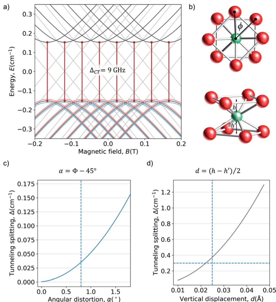
Fig. 5 (a) Zeeman diagrams ( B_z ) for the ground multiplet of HoW 10 with the CF parameters reported in the ESI Section S3† (black lines) and with B_4 parameters that are 2\sigma larger (blue lines) or 2\sigma smaller (red lines), see text for details. Energy origin has been chosen at the center of the anticrossing for convenience. (b) Coordination sphere of HoW 10 , emphasizing the deviation from the ideal D_{4d} symmetry: a skew angle \phi \neq 45^\circ and the off-center position of Ho h \neq h' . (c) Evolution of the calculated tunneling splitting \Delta_{CT} for rising values of angular distortion \alpha . The average crystallographic value is marked with a vertical line. (d) Evolution of \Delta_{CT} for rising values of the vertical displacement d . The averaged crystallographic value is marked with a vertical line and the splitting determined by EPR is marked with a horizontal line.
