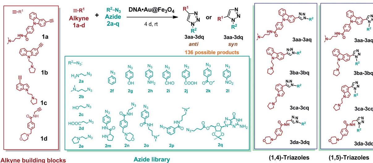
Fig. 3 Alkyne (1a–d) and azide (2a–q) fragments and regiosomeric 1,4- anti (3aa–3dq) and 1,5- syn (3aa–3dq) triazoles derived from combinations of alkyne and azide building blocks.
