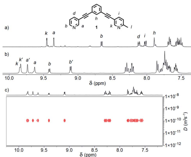
Fig. 2 Partial ^1\text{H} NMR spectra (400 MHz, 298 K) of cages [\text{Pd}_2(\textbf{1})_4](\text{BF}_4)_4 formed in (a) \text{CD}_3\text{CN} , and (b) d_6 -DMSO; (c) ^1\text{H} DOSY spectrum (500 MHz, d_6 -DMSO) of cis - and trans - [\text{Pd}_2(\textbf{1})_4](\text{BF}_4)_4 cage mixture.
