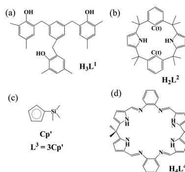
Chart 1 Ligand structures of (a) tris(alkyloxy)arene, (b) trans -calix[2]pyrrole[2]benzene, (c) silylcyclopentadiene, and (d) octadentate Schiff-base polypyrrolic macrocycle.
