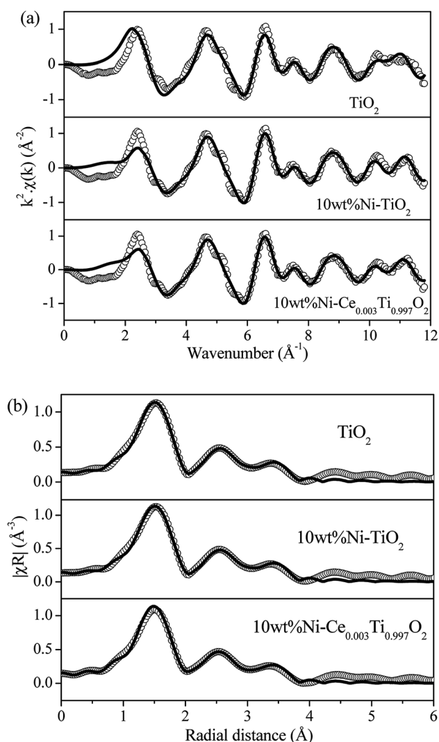
Fig. 5 (a) Experimental (open circle) and calculated (black line) FT-EXAFS spectra in k -space for \text{TiO}_2 , 10 wt% Ni- \text{TiO}_2 and 10 wt% Ni- \text{Ce}_{0.003}\text{Ti}_{0.997}\text{O}_2 . (b) Experimental (open circle) and calculated (black line) FT-EXAFS spectra in R -space for \text{TiO}_2 , 10 wt% Ni- \text{TiO}_2 and 10 wt% Ni- \text{Ce}_{0.003}\text{Ti}_{0.997}\text{O}_2 .
