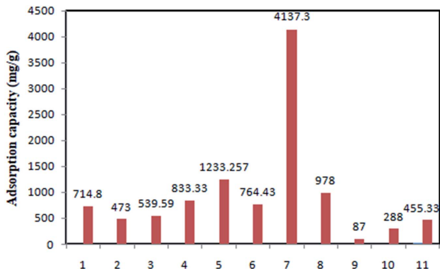
Fig. 5 Comparative evaluation of TC adsorption using different adsorbents [(1) GAC ox 64 (2) MGOS 66 (3) G-KOH 69 (4) Fe 3 O 4 -g-CN@PEI-β-CD 72 (5) TDMGO 73 (6) CoO@C 77 (7) starch-NZV 83 (8) GS-NiFe 124 (9) ferric-activated SBA 87 (10) AC from agricultural residual 130 (11) NaOH-activated AC from macadamia nutshell 129 ].
