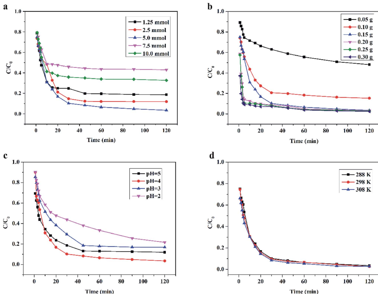
Fig. 5 Effect of different parameters on the degradation of RhB in the heterogeneous catalytic wet peroxide oxidation process: (a) \text{H}_2\text{O}_2 dosage, (b) Ce/PPNW- g -PAA dosage, (c) initial pH, and (d) reaction temperature. Except for the investigated parameter, the other experimental conditions were: initial RhB concentration = 100 \text{ mg L}^{-1} , \text{H}_2\text{O}_2 dosage = 5.0 \text{ mmol} , Ce/PPNW- g -PAA = 0.15 \text{ g L}^{-1} , initial pH = 5.0, and T = 298 \text{ K} .
