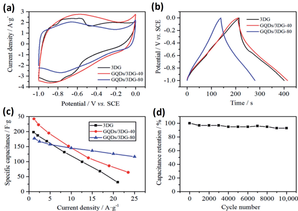
Fig. 18 (a) Cyclic voltammetry curve at a scan rate of 10 mV s -1 (b) charge/discharge curves at different current densities with different compositions, respectively (c) specific capacitance versus current densities and (d) cycling stability at a current density of 24 A g -1 for the composite material. Adapted from ref. 183, copyright 2019, MDPI publications.
