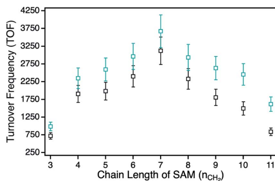
Fig. 4 Photocatalytic ^1\text{O}_2 sensitization activities for the hybrids with a systematic variation of the alkyl chain lengths plotted as function of the SAM chain length. Series H1-3–H1-11 with the peripheral propyloxy-functionalized ZnPc derivative 1 is the cyan trace and series H2-3–H2-11 with peripheral hexyloxy-functionalities (ZnPc 2 ) the black trace.
