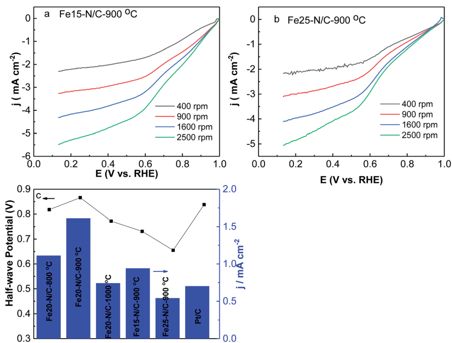
Fig. 9 LSV for oxygen reduction of Fe15-N/C, Fe20-N/C (a), and Fe25-N/C (b) samples fired at 900 °C, Pt/C in O 2 -0.1 M KOH with different rotation speeds with scan rate ( 5 \text{ mV s}^{-1} ). The loading of catalysts was 0.38 \text{ mg cm}^{-2} . Half-wave potential and exchange current density obtained at 0.9 V for Pt/C, Fe20-N/C samples fired at 800 °C, 900 °C, 1000 °C and Fe15-N/C, Fe20-N/C, and Fe25-N/C samples fired at 900 °C (c).
