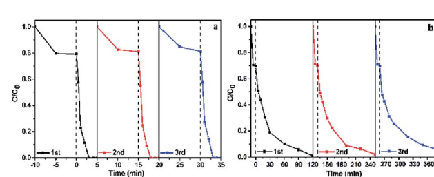
Fig. 10 Cycling runs of the as-prepared rGO/GNW for adsorption and photocatalytic degradation of ethenzamide under VUV (a) and UV (b) light irradiation.
