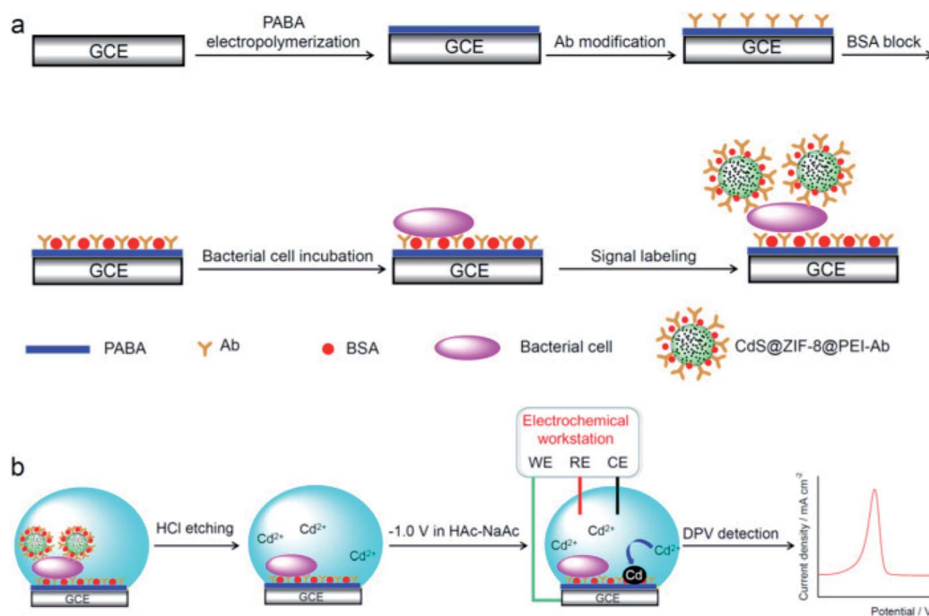
Fig. 8 (a) Fabrication of sandwiched electrochemical immunosensor for detection of E. coli : GCE was modified with poly( p -aminobenzoic acid) (PABA) followed by anti- E. coli O157:H7 Ab covalent immobilization, blocking with bovine serum albumin (BSA), E. coli incubation and finally labelling with CdS@ZIF-8@PEI-Ab tags. (b) Electrochemical detection of leached Cd(II) resulting from etching of CdS@ZIF-8@PEI-Ab tag. Adapted from ref. 78 with permission from Elsevier B.V., Copyright 2018.
