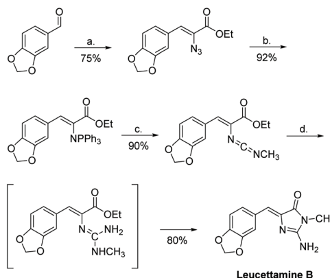
Scheme 46 The first total synthesis of leucettamine B. Reagents (a) \text{N}_3\text{CH}_2\text{COOEt} , \text{NaOEt} , -15\text{ }^\circ\text{C} ; (b) \text{Ph}_3\text{P} , \text{CH}_2\text{Cl}_2 , rt; (c) \text{CH}_3\text{NCO} , toluene, rt; (d) \text{NH}_3 , sealed tube, 45\text{ }^\circ\text{C} .
