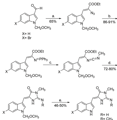
Scheme 30 Iminophosphorane-mediated ring formation to produce (Z)-aplysinsopins derivatives. Reagents: (a) \text{N}_3\text{CH}_2\text{COOC}_2\text{H}_5 , NaOEt, EtOH, -15^\circ\text{C} , (b) \text{PPh}_3 , \text{CH}_2\text{Cl}_2 , rt, (c) \text{CH}_3\text{-NCO} , toluene, rt, (d) \text{NH}_2\text{R} , toluene, 45^\circ\text{C} , (e) \text{HCOOH} , reflux.
