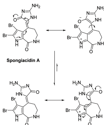
Scheme 42 Isomerization of ( E )-spongiacidin A to the ( Z )-isomer.
