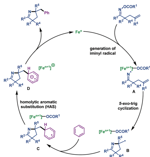
Scheme 14 Okamoto and Ohe's iron-catalyzed imino-arylation of \gamma,\delta -unsaturated oxime esters with arenes.
