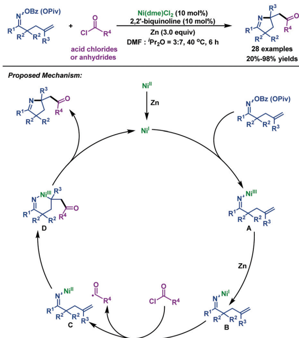
Scheme 43 Wang's nickel-catalyzed imino-acylation of \gamma,\delta -unsaturated oxime esters with acid chlorides or anhydrides.
