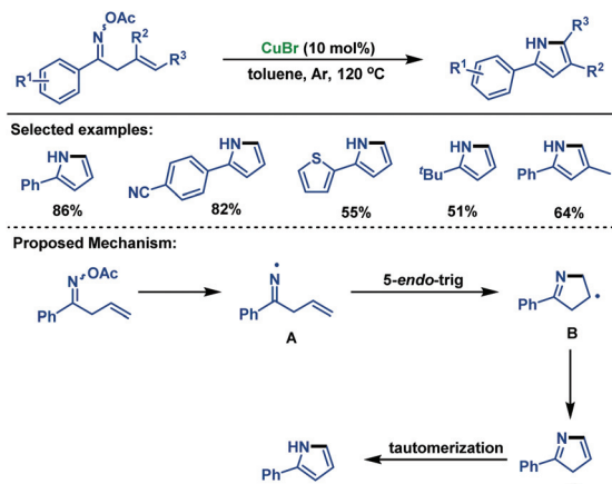
Scheme 53 Guan's copper-catalyzed 5-endo-trig cyclization of \beta,\gamma -unsaturated oxime esters for the synthesis of pyrroles.
