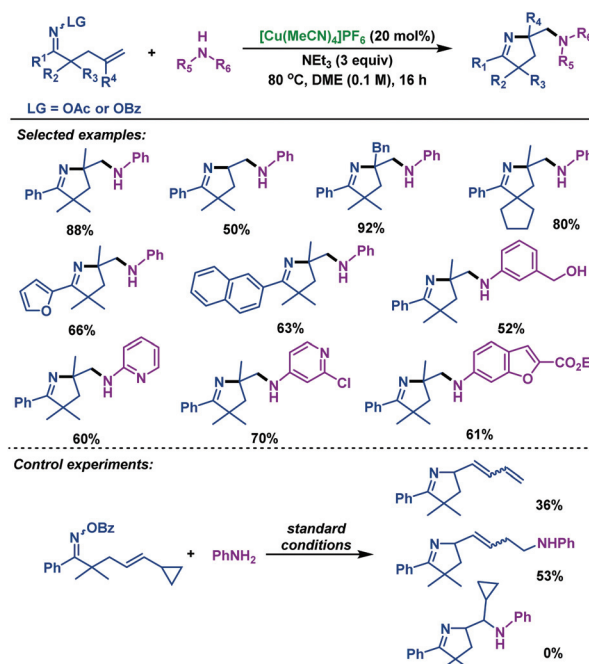
Scheme 12 Wang's copper-catalyzed diamination of \gamma,\delta -unsaturated oxime esters with unprotected amines.
