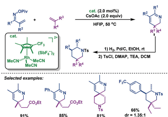
Scheme 49 Rovis' Rh(III)-catalyzed coupling of \alpha,\beta -unsaturated oxime esters with 1,1-disubstituted alkenes for the synthesis of 2,3-dihydropyridines.
