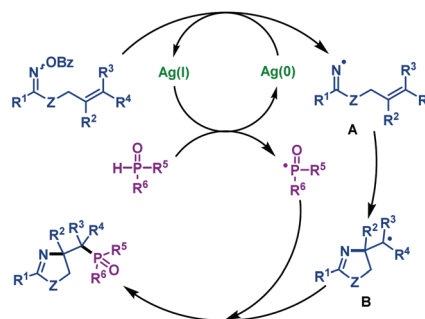
Scheme 20 Proposed mechanism.
