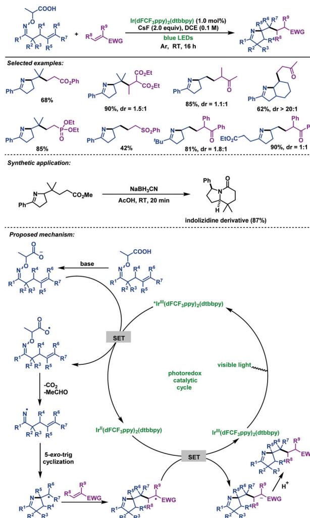
Scheme 25 Studer's visible-light-promoted carboimination of \gamma,\delta -unsaturated oxime ethers with Michael acceptors.
