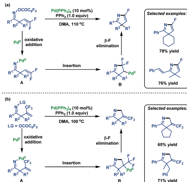
Scheme 46 Ichikawa's palladium-catalyzed intramolecular Heck-type 5- endo-trig cyclization of \beta,\gamma -unsaturated oxime esters.
