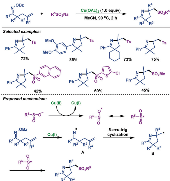
Scheme 8 Zhu and Chen's copper-promoted imino-sulfonylation of \gamma,\delta -unsaturated oxime esters with sodium sulfinates.
