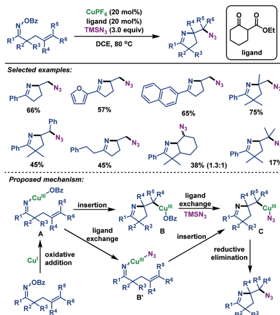
Scheme 44 Yu's copper-catalyzed imino-azidation of \gamma,\delta -unsaturated oxime esters with \text{TMSN}_3 .
