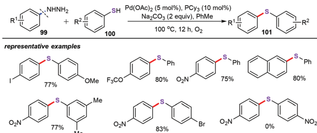
Scheme 37 Palladium-catalyzed oxidative cross-coupling of arylhydrazines with arenethiols.
