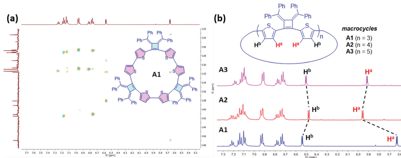
Fig. 3 Structural elucidation of Macrocycles A1 , A2 and A3 by NMR spectroscopy. (a) 2D NMR HMBC (500 MHz, 25 °C, THF- d 8 ) spectrum of A1 . (b) 1 H NMR (500 MHz, 25 °C, THF- d 8 ) spectra of A1 , A2 and A3 .
