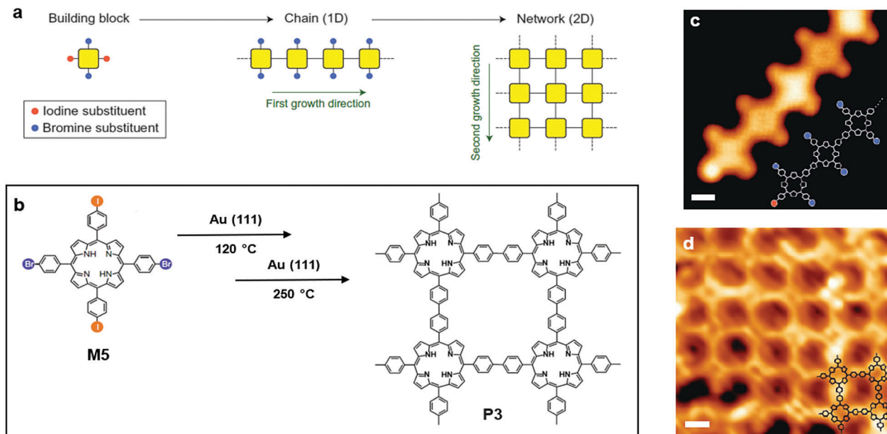
Fig. 5 (a) Schematic illustration of polymerization (two steps) onto the solid surface of Au(111). (b) Chemical structure of 5,15-bis(4-bromophenyl)-10,20-bis(4-iodophenyl)porphyrin ( trans -Br212TPP) ( M5 ) and polymer3 ( P3 ). (c) STM image of the chain formed by M5 (scale bar 1 nm). (d) STM image of P3 (scale bar 1 nm). Reprinted with permission from ref. 55, Copyright 2012, Nature Publishing Group.
